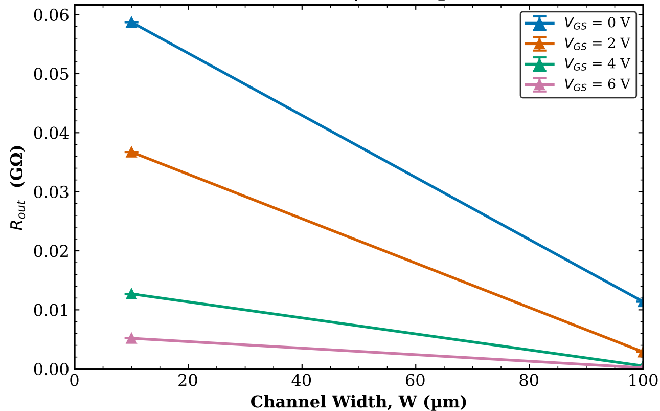
TFT3 Transistor 2 R_{out} vs W | L = 8\text{ }\mu\text{m}
